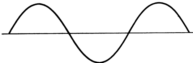
Figure 7-1. Sine Wave
