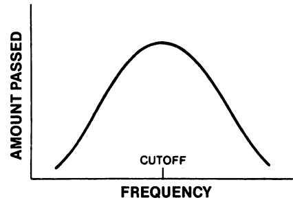
Figure 7-9. Band-pass Filter
