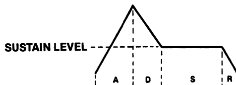
Figure 7-4. ADSR Phases
