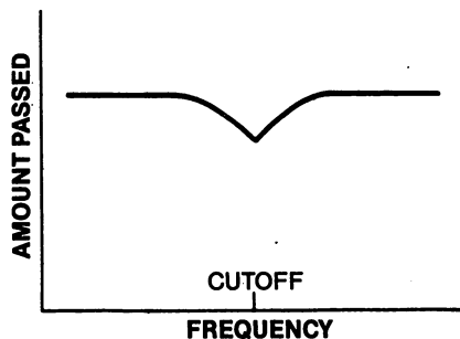
Figure 7-10. Notch Reject Filter
